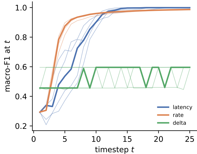
ctu13_v2_f0: evidence accumulation (per seed)
