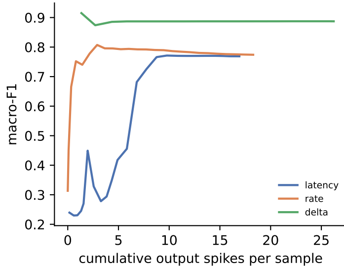
quality vs temporal cost (median)
