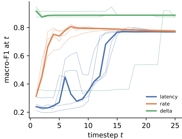
ctu13_v2_f1: evidence accumulation (per seed)
