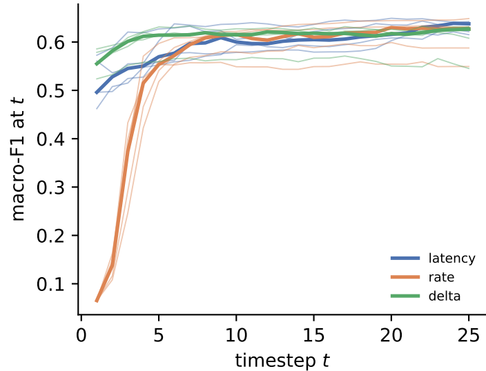
kddcup99_v2: evidence accumulation (per seed)
