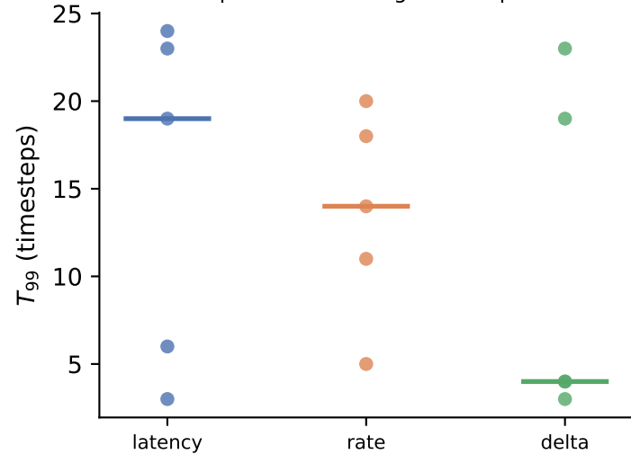
per-seed convergence step
