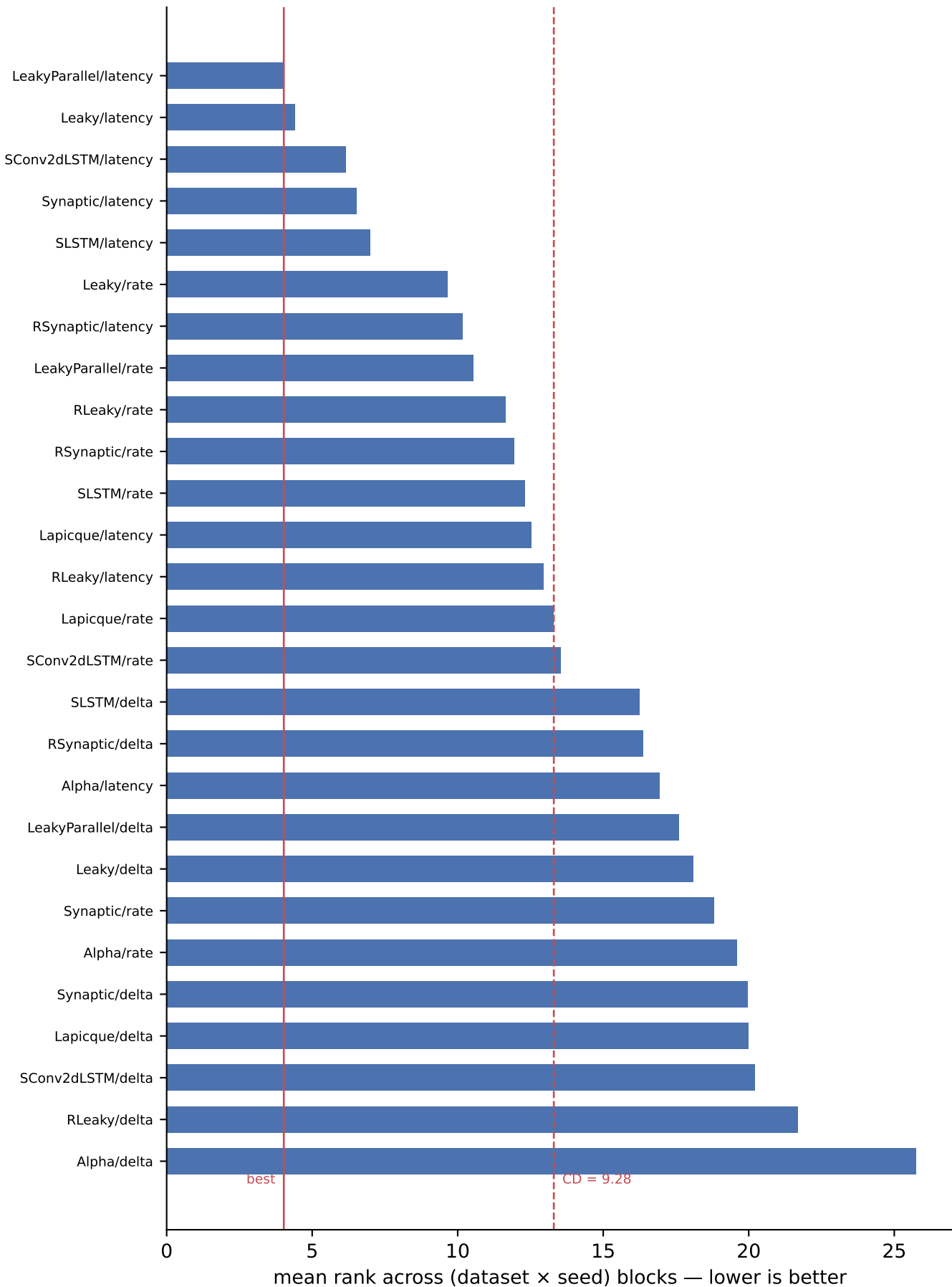
v1: f1_macro, 27 variants over 20 blocks
