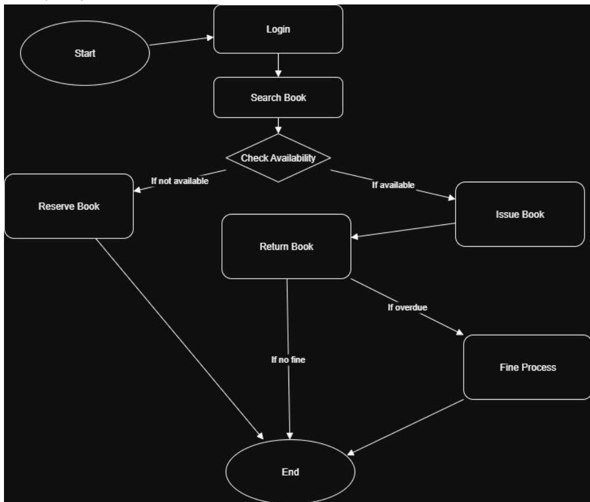
Activity Diagram:
