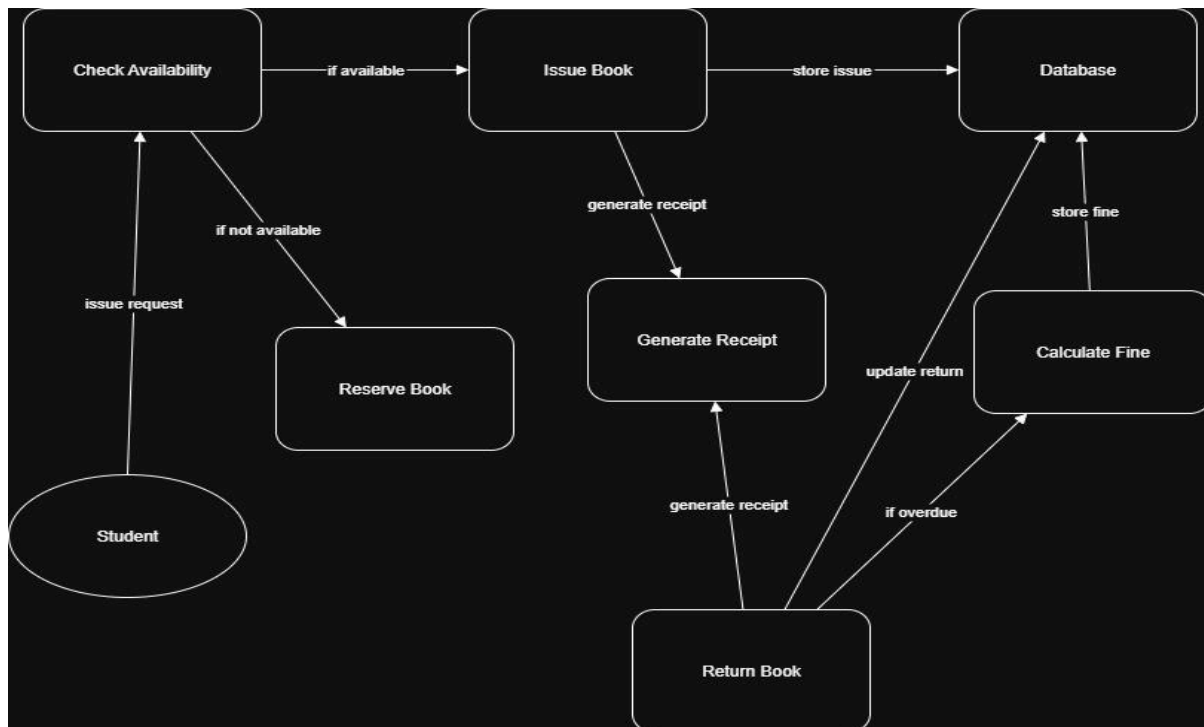
USE-CASE Diagram:
