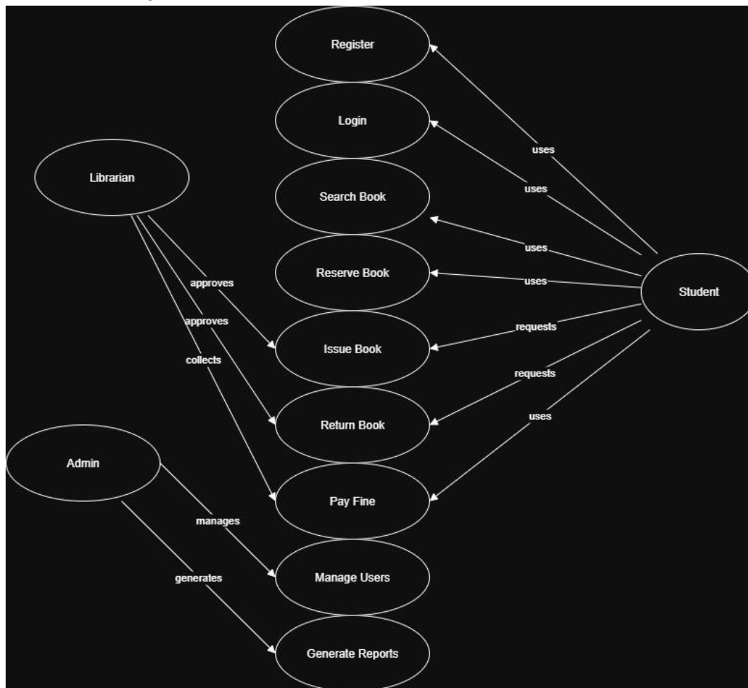
USE-CASE Diagram:
