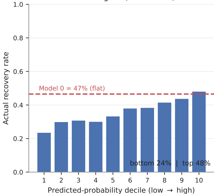
Chronological (out-of-time)
