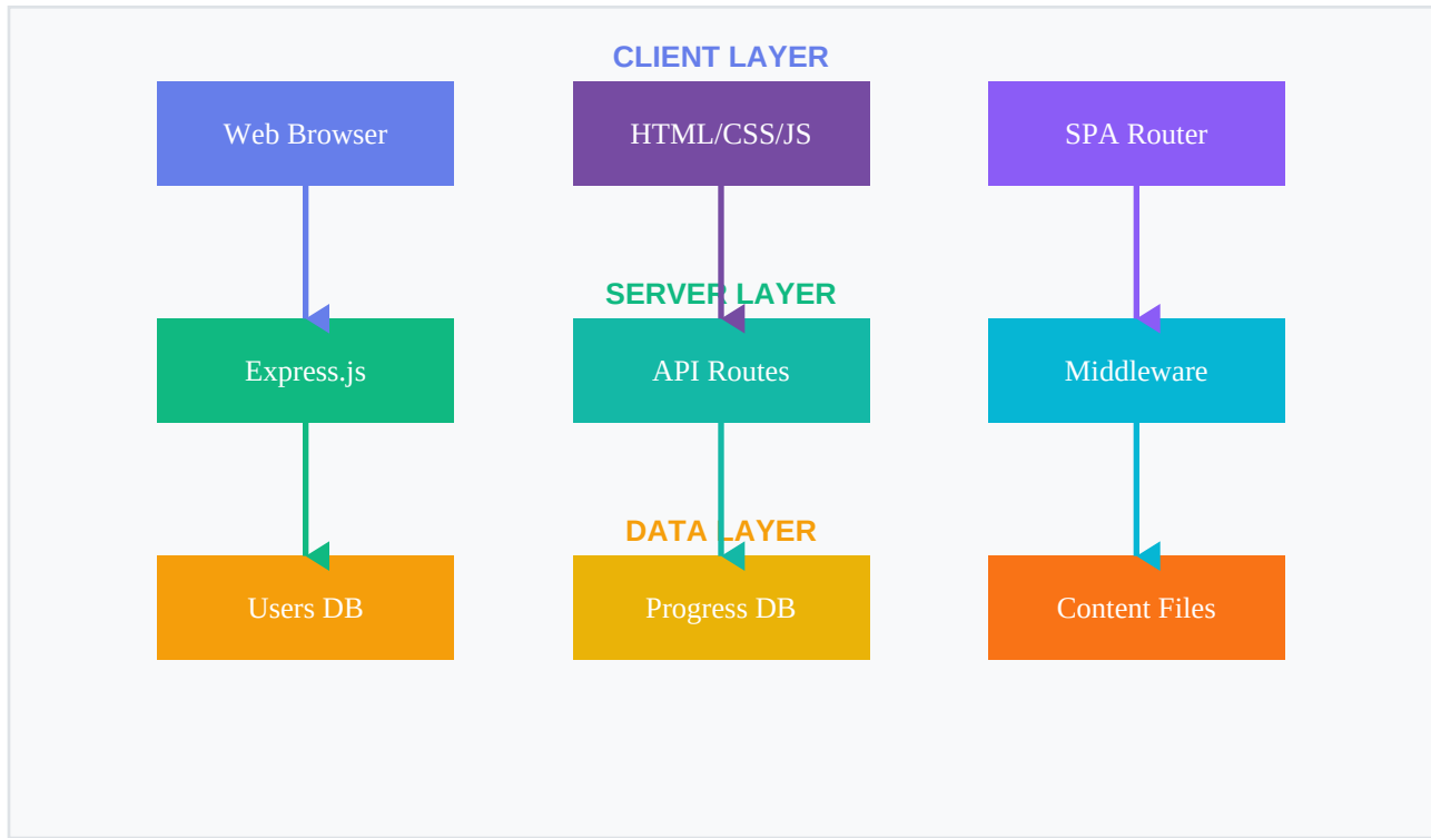
Figure 1: System Architecture - Three-tier architecture with Client, Server, and Data layers
