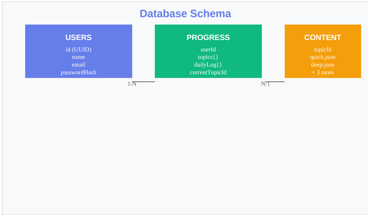
Figure 4: Database schema showing users, progress, and content relationships
