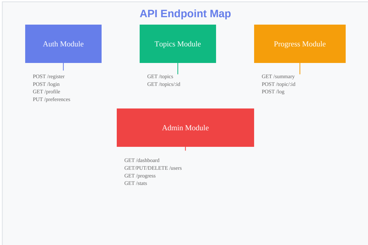
Figure 7: API endpoints organized by functional module
