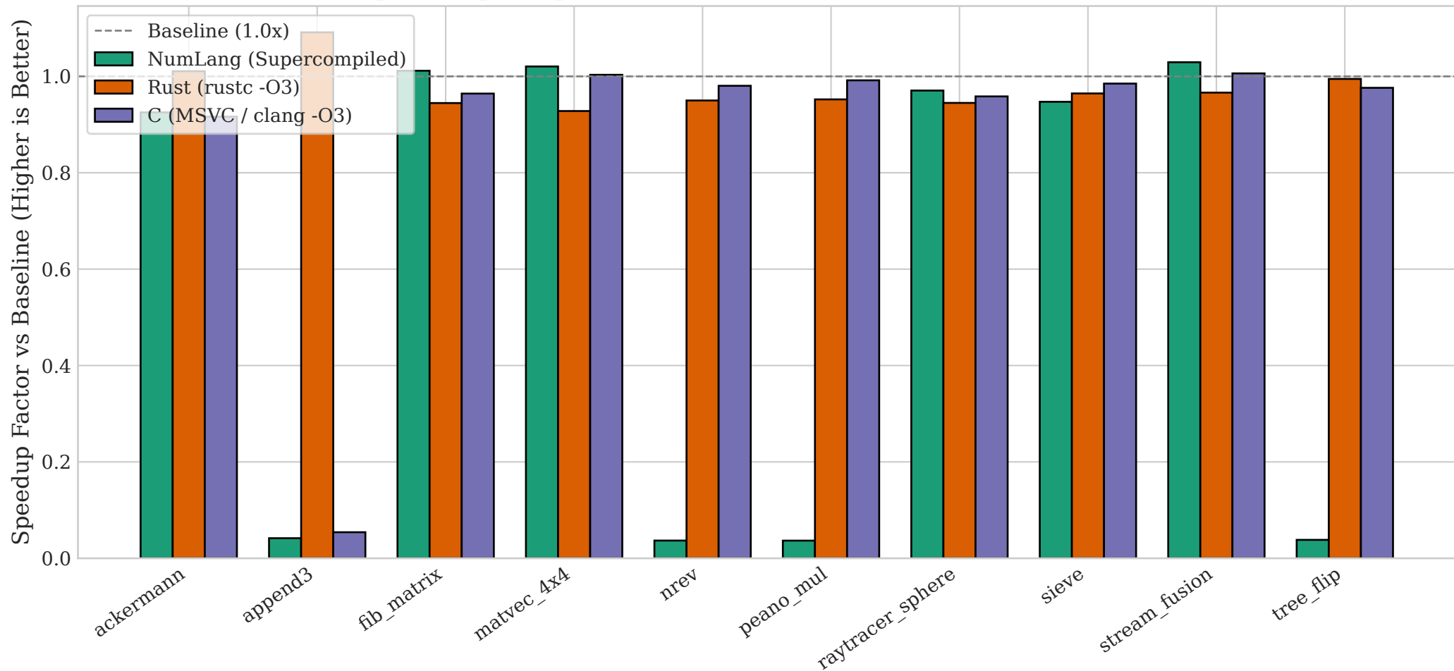
Empirical Speedup on Literature Benchmark Suite (Geometric Mean)
