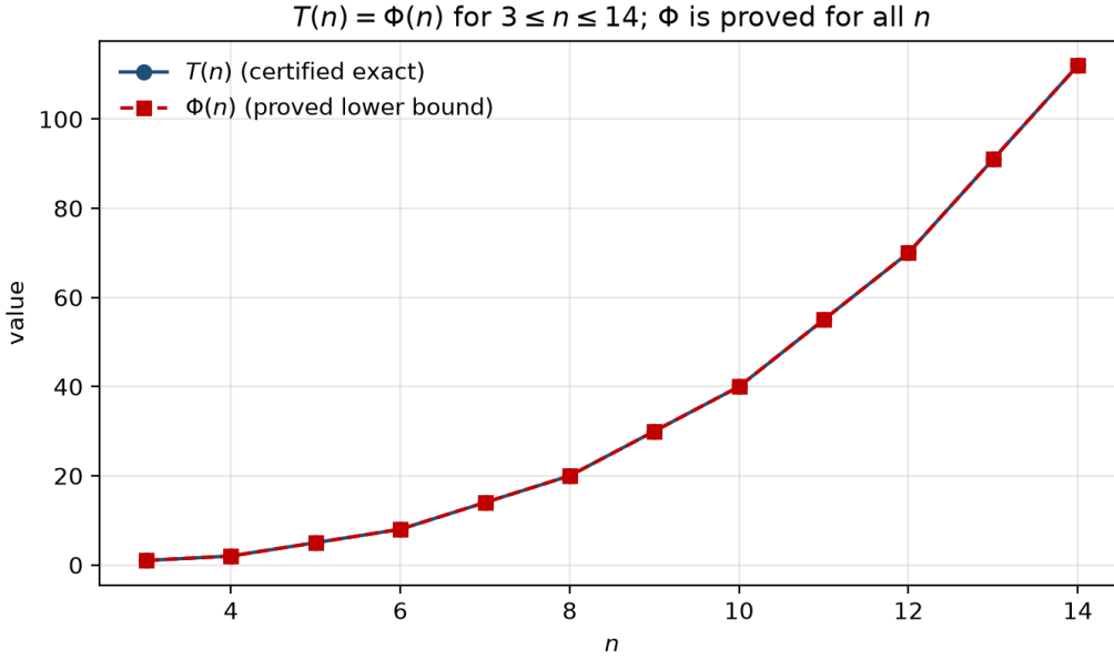
Figure 1: The exact values coincide with the proved lower bound wherever we can compute them (Theorem 6.1).
