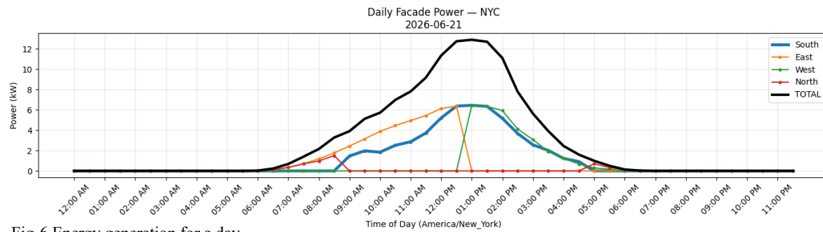
Fig-6 Energy generation for a day
