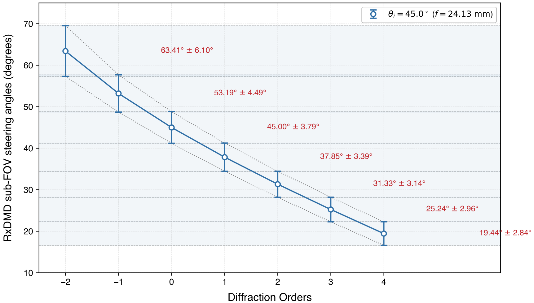
RxDMD sub-FOV Steering Angles vs. Diffraction Orders
