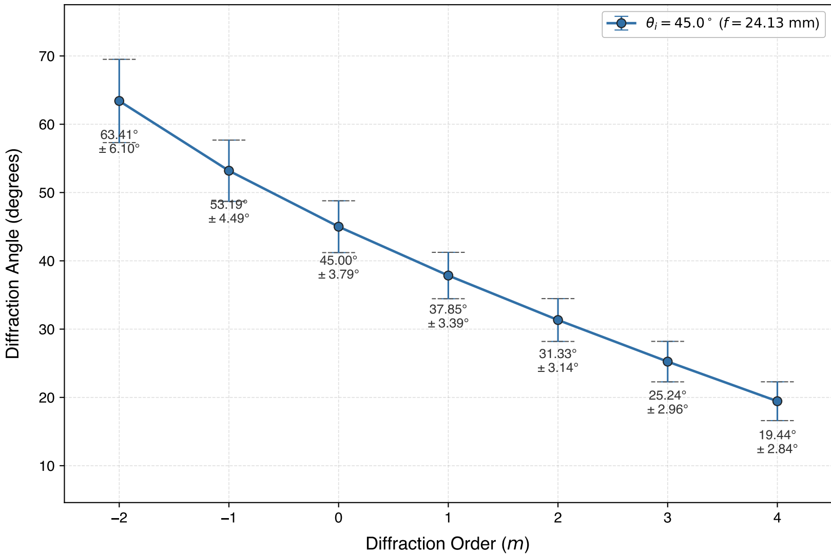
RxDMD Steering Angles vs. Diffraction Orders
