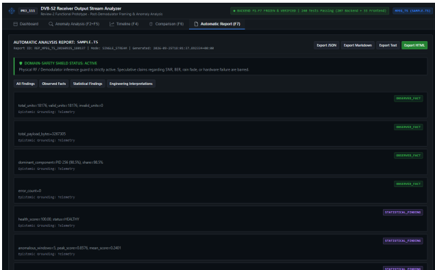
Fig. 6. Multi-format diagnostic report generation view (Feature F7) showing tripartite findings categorization and one-click export controls.
