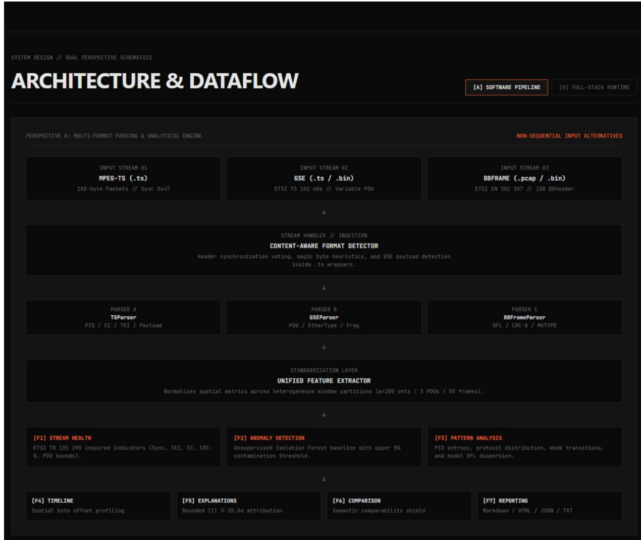
Fig. 1. End-to-End Architectural Pipeline of the PRJ_111 DVB-S2 Receiver Output Stream Analyzer (Stages 1 through 6).
