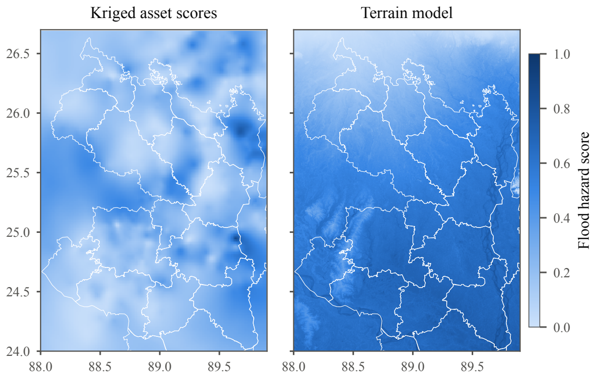
Figure S1: The two flood hazard surfaces for Rangpur and Rajshahi, with district boundaries in white. The Kriged surface interpolates the asset model’s scores between mapped assets and has a standard deviation of 0.13 across the grid. The terrain model scores each 30 m cell from its own elevation, slope, TWI, HAND and flow accumulation, has a standard deviation of 0.24, and reaches a cell-level AUC against observed flooding of 0.657, against 0.666 for the Kriged surface.
