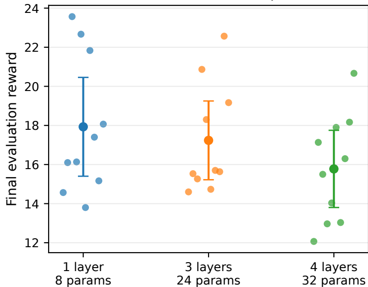
Reward vs circuit depth
