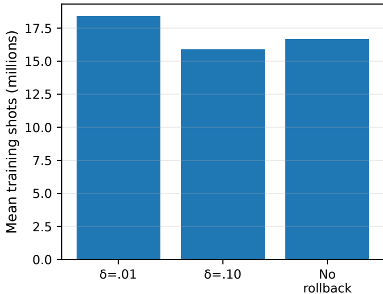
Quantum measurement cost
