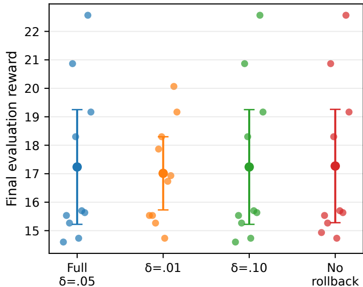
Reward
