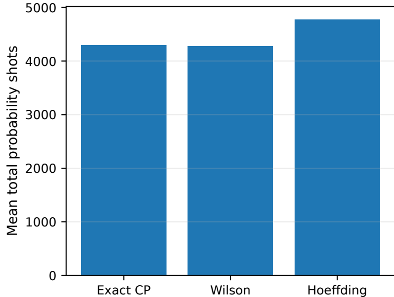
Measurement cost
