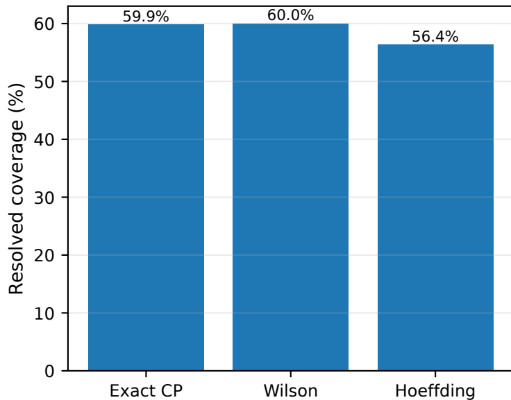
Decision coverage
