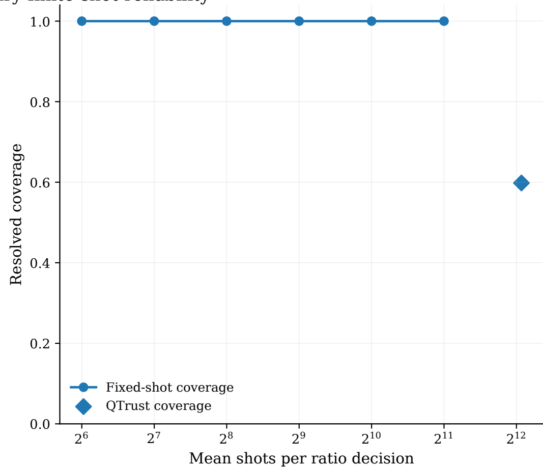
Controlled near-boundary finite-shot reliability
