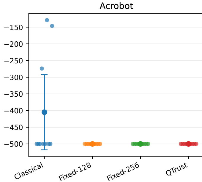
Main benchmark across ten training seeds
