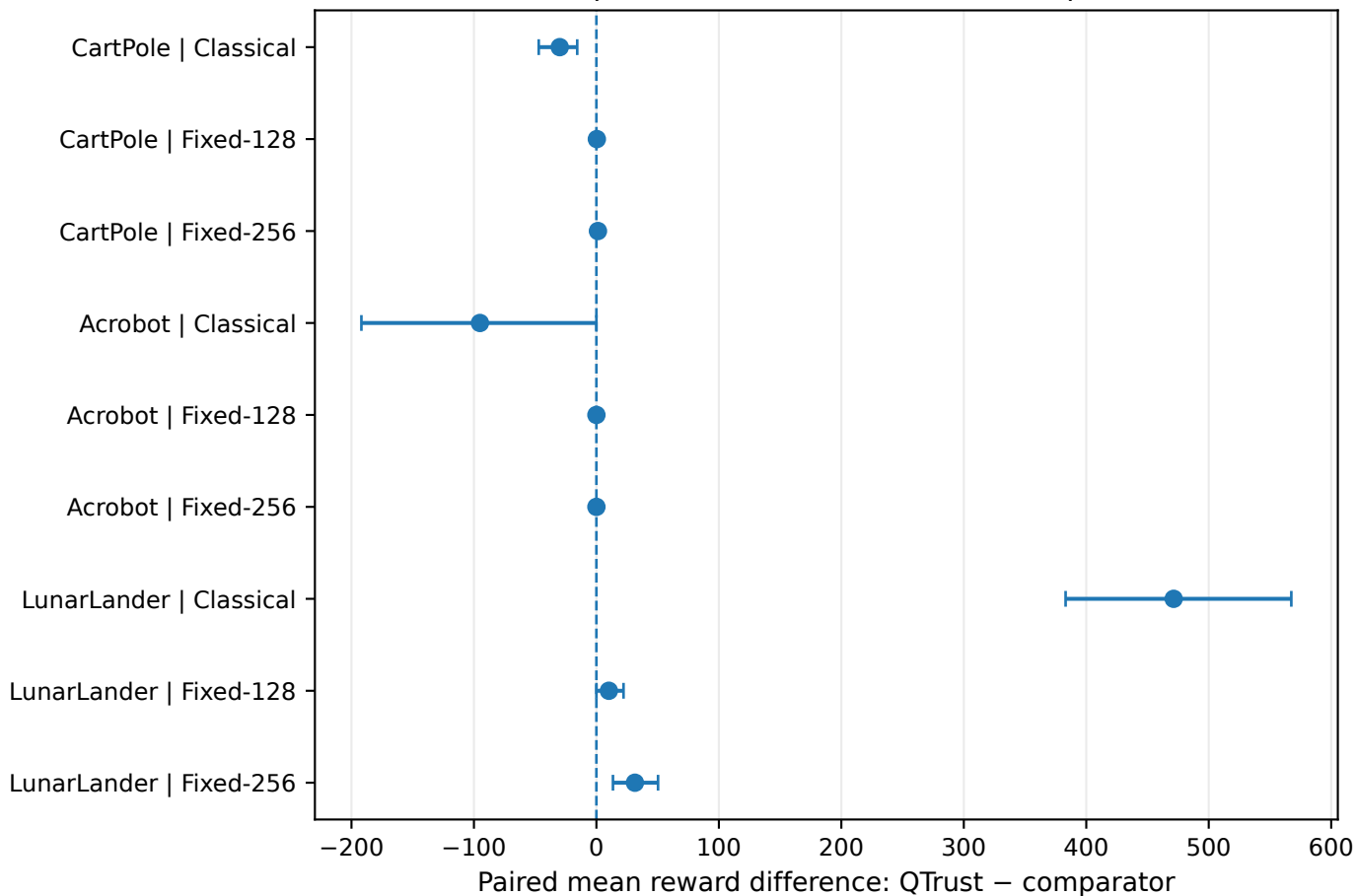
Main paired effects with 95% bootstrap CIs
