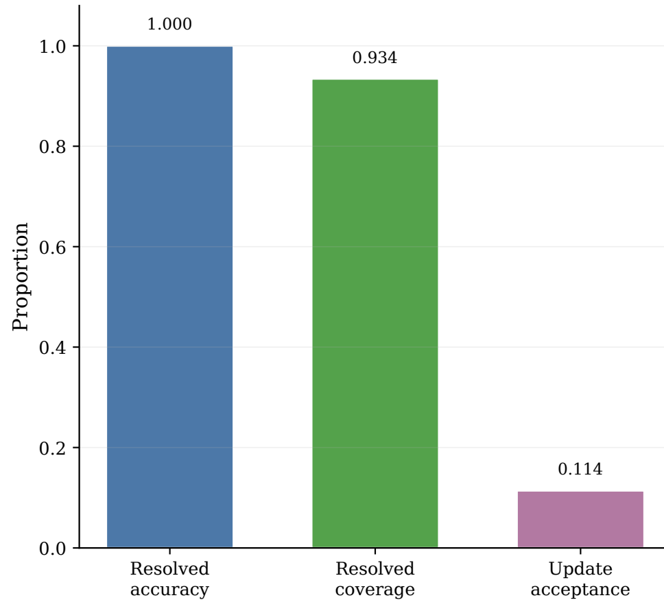
QTrust certification reliability and update gating Acrobot-v1
