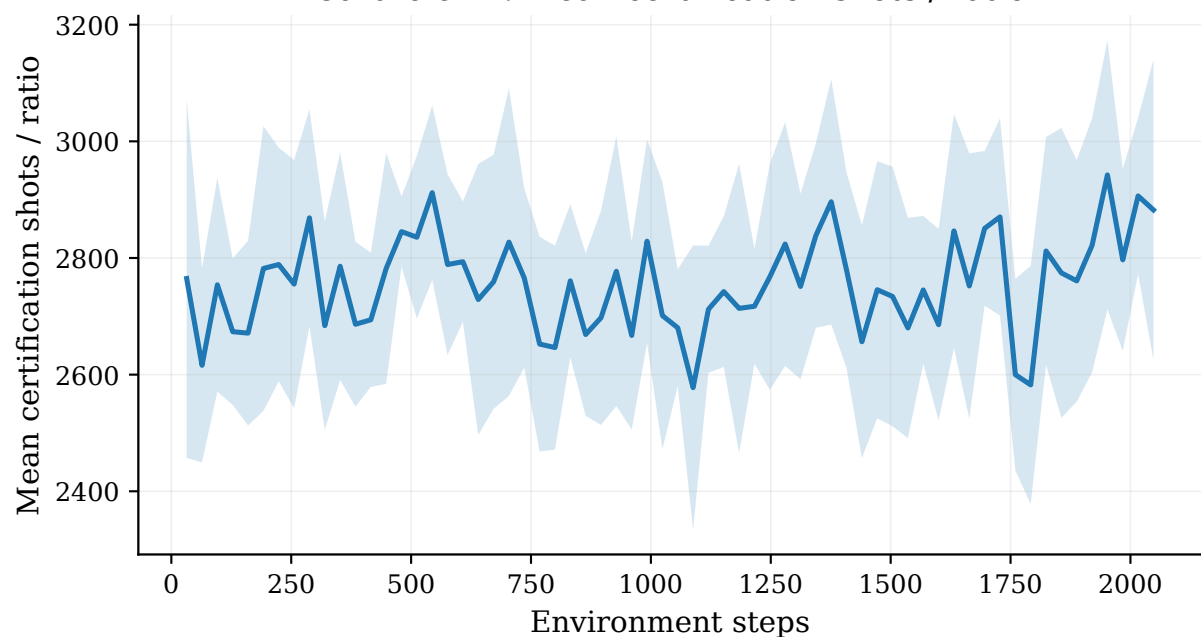
QTrust training dynamics across 10 independent seeds (mean \pm 95% t-CI)
