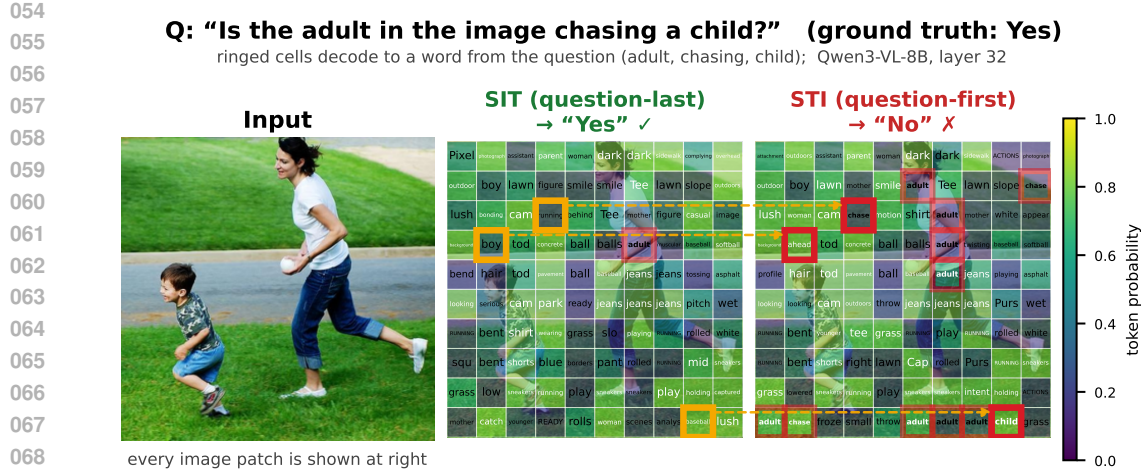
Figure 1: The ordering that looks most like it found the answer is the one that answers wrong. Every image patch of one NaturalBench example is shown, each cell holding the vocabulary token that patch’s layer-32 hidden state decodes to under a logit lens, shaded by that token’s probability. Moving the question in front of the image steers the patches onto the question’s own vocabulary, taking patches that decode a question word from 1 to 12 (red rings), yet the model then answers “No” to a question whose ground truth is Yes, while question-last answers “Yes”. Amber boxes mark three traced patches, joined by a dashed arrow to the same patch under question-first, where it is boxed in red: running becomes chase , boy becomes ahead , baseball becomes child . Better perception, worse answer. Echoing the question after the image keeps all 12 steered patches and recovers the answer for 13 tokens.
