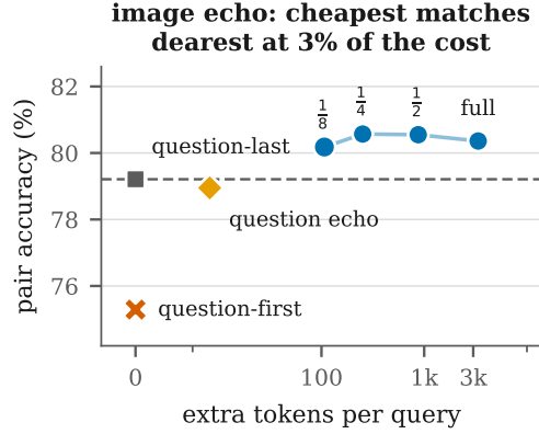
Figure 2: Accuracy is flat across a 31\times range of echo cost, so the cheapest echo is the one to ship. Cost against accuracy on NaturalBench; the x axis is extra tokens per query relative to question-first, on a symmetric log scale so that 0 can be shown. The dashed line is the question-last baseline, which every image echo clears. The \frac{1}{8} -resolution echo (+107 tokens) is statistically indistinguishable from the full-resolution one (+3,352).
