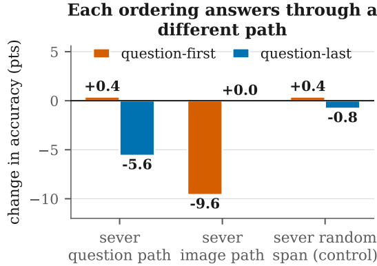
Figure 5: Each ordering answers through a different path. Bars are the change in accuracy against the unmodified run (57.6 for question-first, 58.8 for question-last). Severing answer-to-question hurts only question-last; severing answer-to-image hurts only question-first; the random span-size control moves both by at most 0.8 points.
