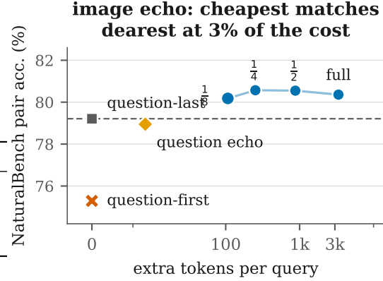
Figure 4: Cost against accuracy on NaturalBench. The x axis is extra tokens per query versus question-first (symmetric log, so 0 is shown); the dashed line is question-last. Every image echo clears that baseline, and the \frac{1}{8} -resolution echo (+107 tokens) is indistinguishable from the full one (+3,352).
