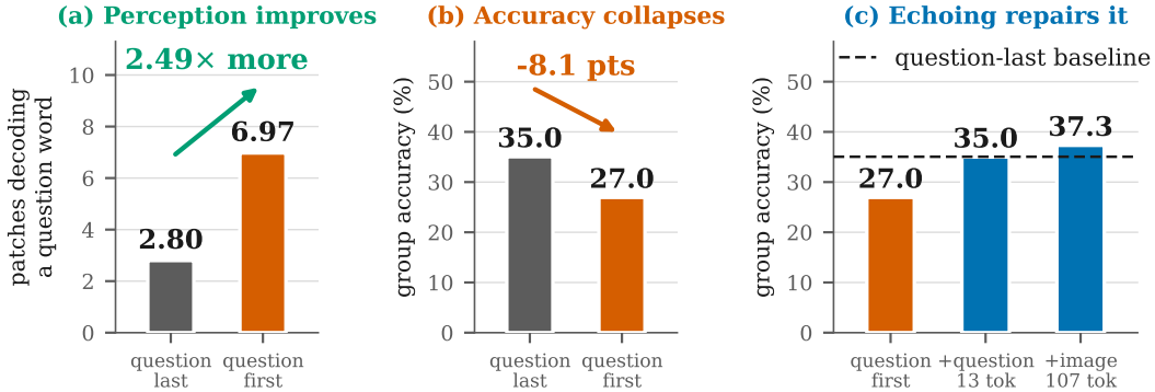
Figure 1: The question-first paradox and its repair, Qwen3-VL-8B. (a) Question-first makes 2.49\times more image patches decode a question content word (160 NaturalBench candidates), so the question reaches the image. (b) It still loses 8.1 points of group accuracy ( p = 1.3 \times 10^{-12} ). (c) Echoing the question after the image repairs it for 13 tokens; an \frac{1}{8} -resolution image echo beats the baseline for 107.
