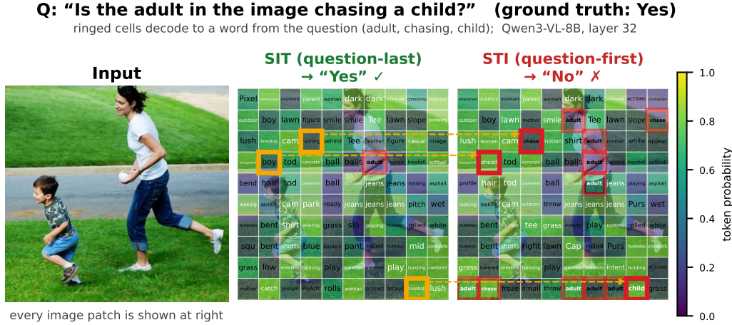
Figure 2: Steering happens, and is not read out. Every image patch is shown: each cell holds the vocabulary token that patch’s layer-32 hidden state decodes to under the logit lens, shaded by that token’s probability. Red rings mark patches decoding a word from the question. Question-last leaves the patches generic (1 ringed patch) and answers correctly; question-first steers the same patches onto the question’s vocabulary (12 ringed patches) and answers wrong. Amber boxes mark three individual patches in the question-last panel, joined by a dashed arrow to the same patch in the question-first panel, where it is boxed in red: running becomes chase , boy becomes ahead , and baseball becomes child . Echoing the question keeps all 12 steered patches and answers correctly again.
