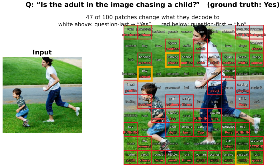
Figure 1: The ordering that looks most like it found the answer is the one that answers wrong. Every image patch of one NaturalBench example is shown once, carrying the vocabulary token it decodes to under a logit lens at layer 32. Unchanged patches carry one dimmed token; changed patches are outlined and carry both, question-last above in white and question-first below in red, with amber outlines on three of them ( running to chase , boy to ahead , baseball to child ). Moving the question in front of the image changes 47 of the 100 patches and takes the count decoding a word from the question itself from 1 to 12, yet the model then answers “No” where the ground truth is Yes and question-last answers “Yes”. Better perception, worse answer. Echoing the question after the image keeps all 12 steered patches and recovers the answer for 13 tokens.
