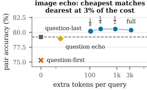
Figure 2: Accuracy is flat across a 31\times range of echo cost, so the cheapest echo is the one to ship. NaturalBench; x is extra tokens per query against question-first, symmetric log so 0 shows. Every image echo clears the question-last baseline (dashed), and the \frac{1}{8} echo (+107 tokens) is indistinguishable from the full one (+3,352).
