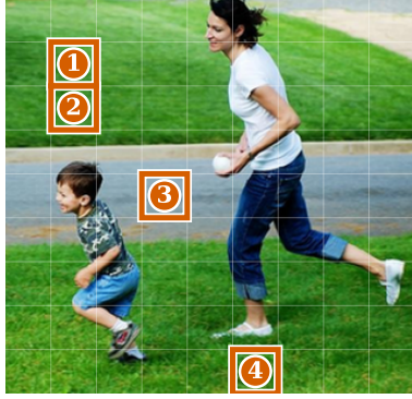
Figure 2: The question rewrites what the image patches say, and the model still answers wrong. NaturalBench example 1007, logit-lens top-1 token per patch at layer 32 over a 9 \times 9 grid; question-first changes 46 of the 81 patch words and four are called out. Scene vocabulary ( boy , hand , throws , woman ) becomes the question’s own vocabulary ( toddler , ahead , chase , adult ), including the answer word, yet question-first answers “No” to a question whose ground truth is Yes. Patch decodes are not localized to the object they name.
