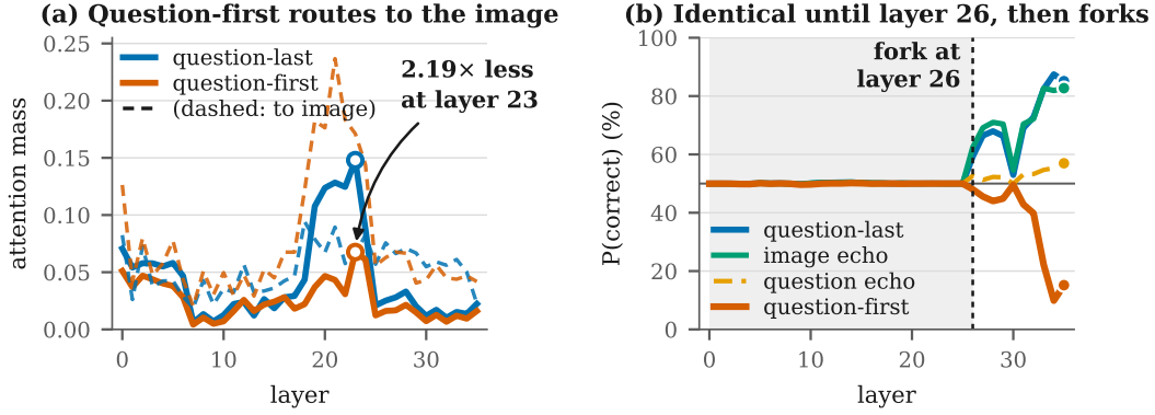
Figure 3: Question-first answers by reading the image instead of the question, and the two orderings only part company in the last quarter of the network. Measured on the 150 NaturalBench pairs where question-first is wrong and question-last is right. (a) Attention mass leaving the answer position, to the question (solid lines) and to the image (dashed): at layer 23, where question attention peaks for both, question-first sends 2.19\times less of it to the question. (b) Probability of the correct answer at each layer. Both baselines sit at chance through layer 25 (shaded), fork at layer 26 and never re-cross; both echo orderings track question-last, not question-first.
