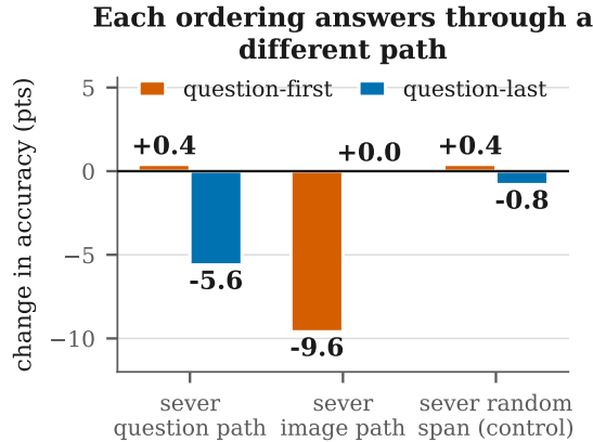
Figure 5: Each ordering answers through a different path, and cutting the other one costs it nothing. Bars are the change in accuracy against the unmodified run (57.6 for question-first, 58.8 for question-last), so downward is damage. Severing answer-to-question hurts only question-last; severing answer-to-image hurts only question-first; severing a random pre-image span of equal length, the control for simply removing attention mass, moves both by at most 0.8 points.
