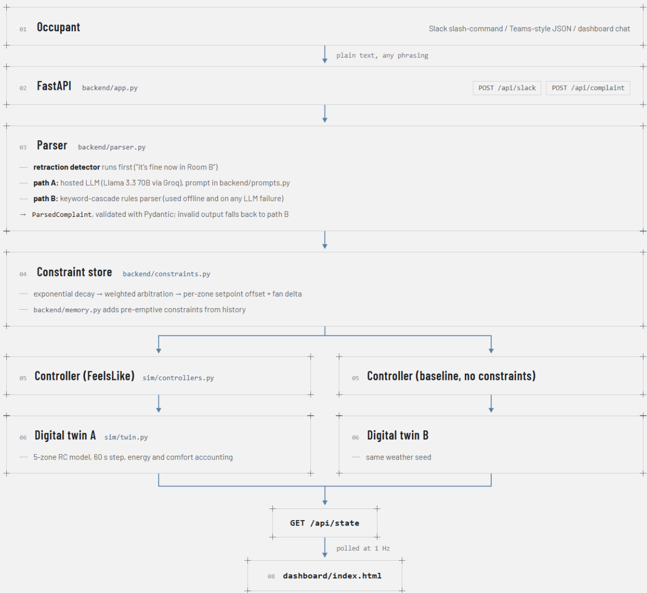
FIG. 01 SYSTEM FLOWCHART
