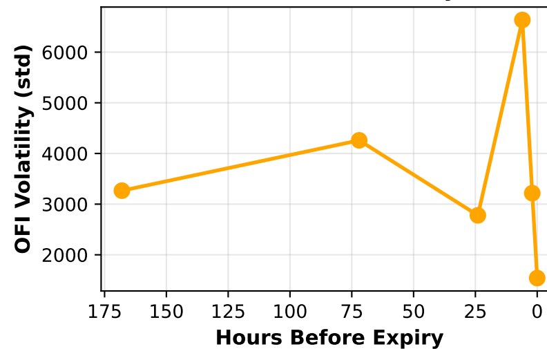
Hours Before Expiry Order Flow Volatility
