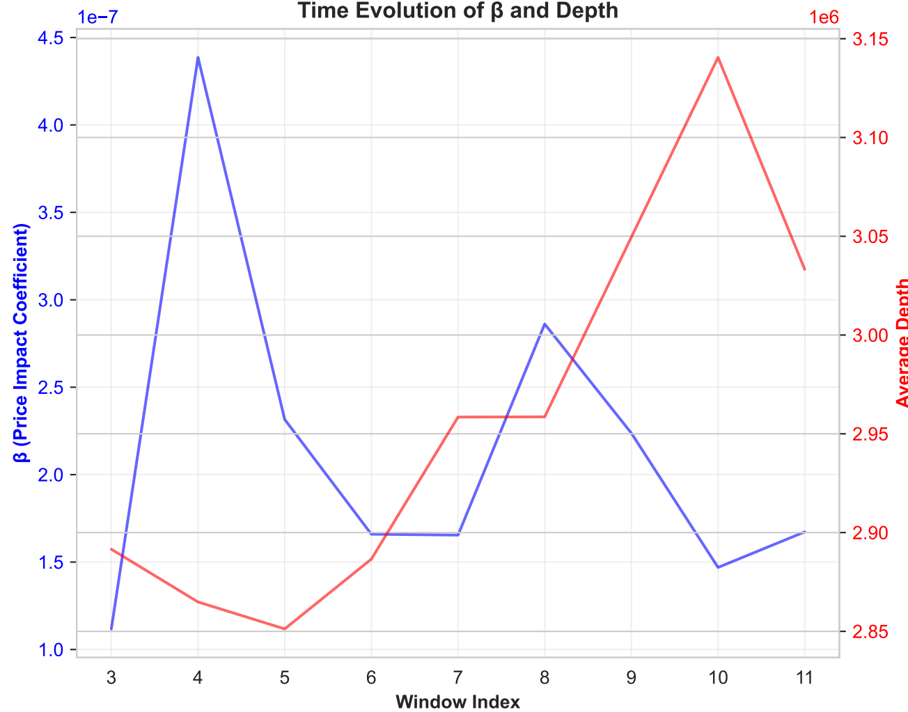
Fed Market Power Law: \beta \propto 1/AD^\lambda
