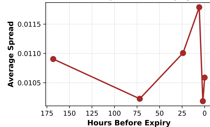
Hours Before Expiry Bid-Ask Spread Near Expiry
