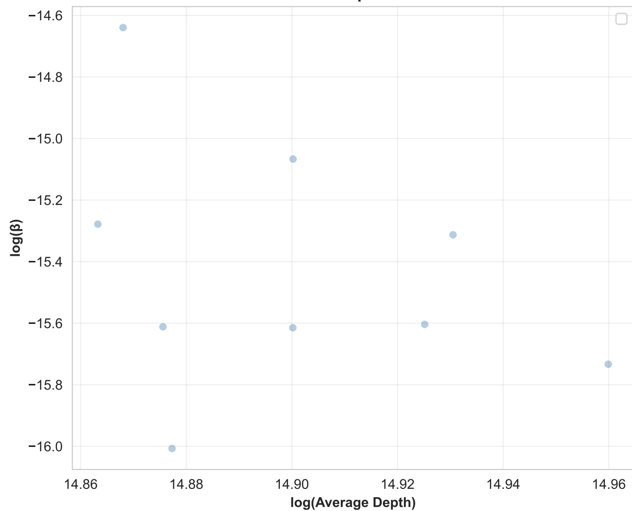
Fed Market Power Law: \beta \propto 1/AD^\lambda
