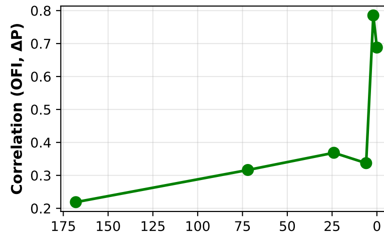
Hours Before Expiry Order Flow Volatility
