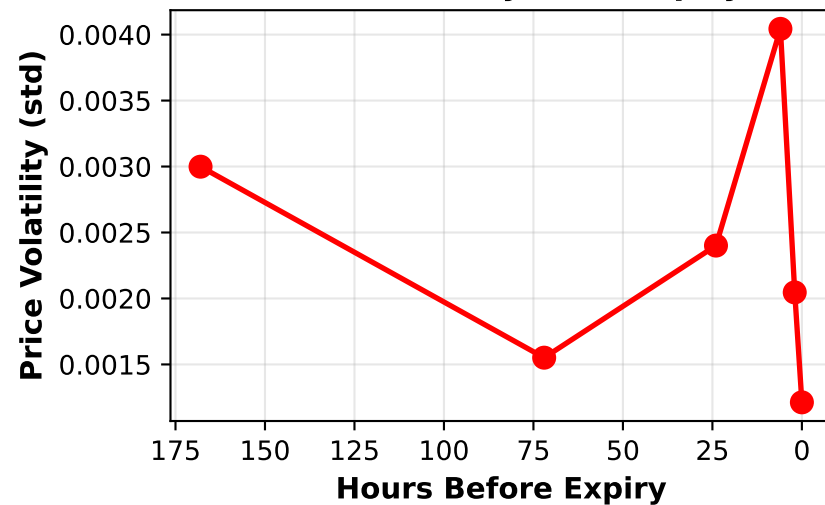
Hours Before Expiry Price Volatility Near Expiry
