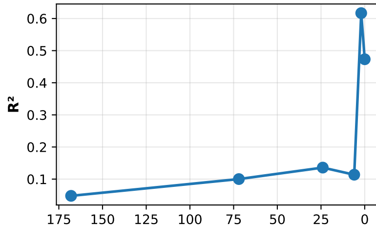
Hours Before Expiry Price Volatility Near Expiry
