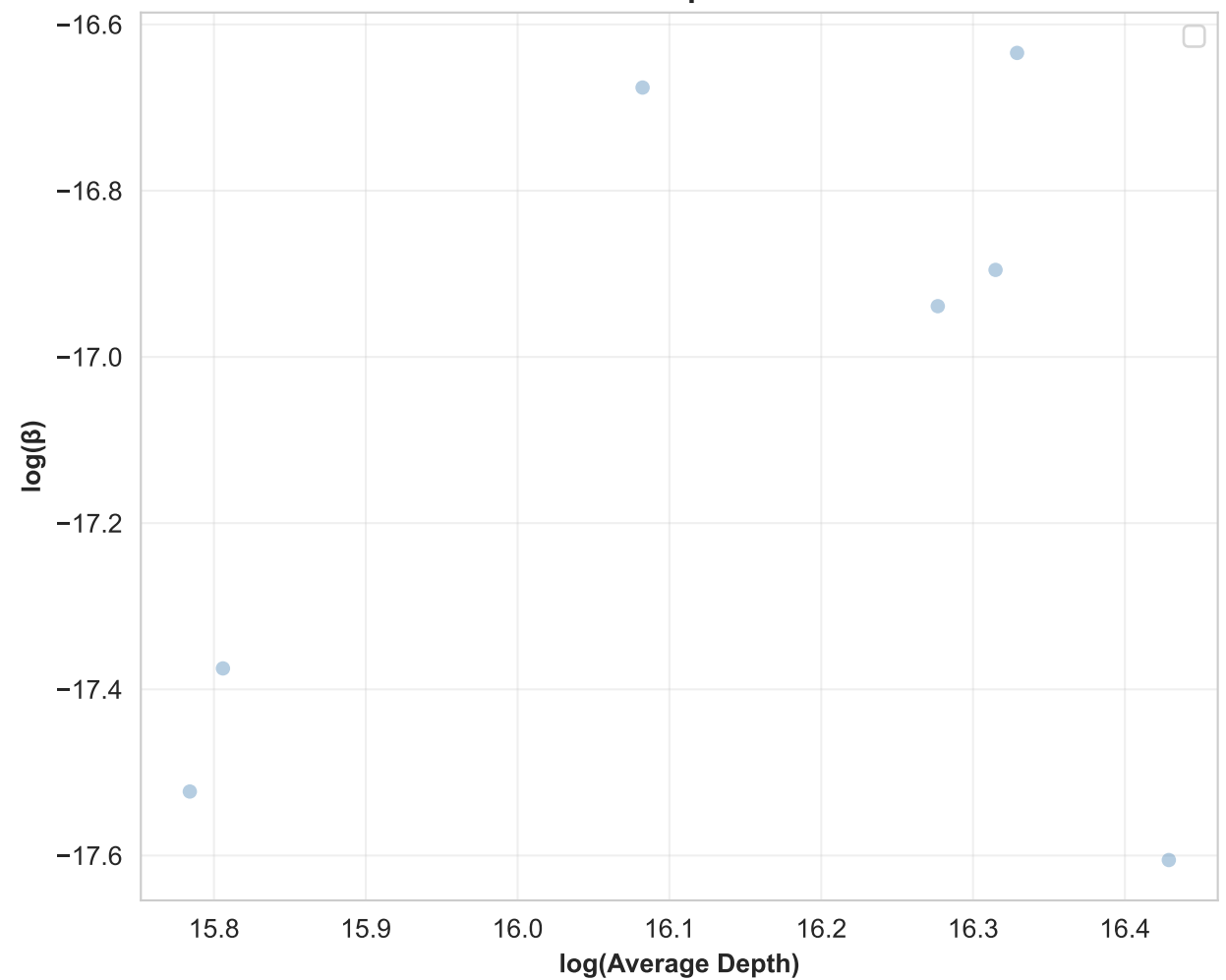
NYC Market Power Law: \beta \propto 1/AD^\lambda
