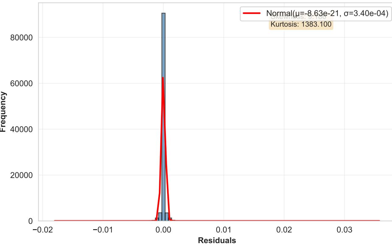
Distribution of Residuals (Check for Normality)
