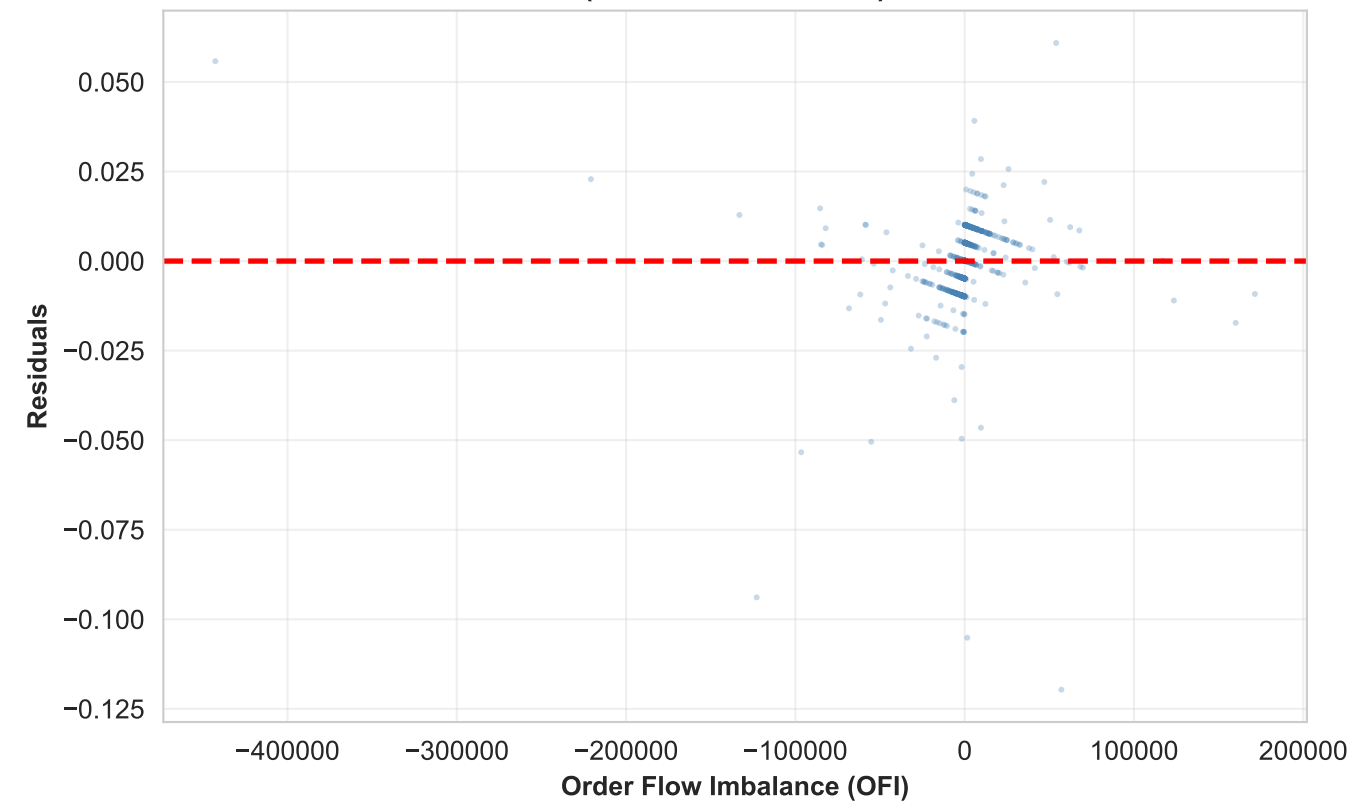
Residuals vs OFI (Check for Patterns)
