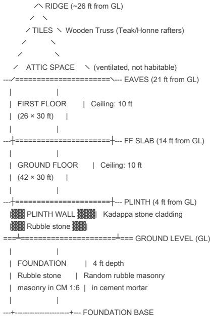
SECTION A-A' (Looking East)
