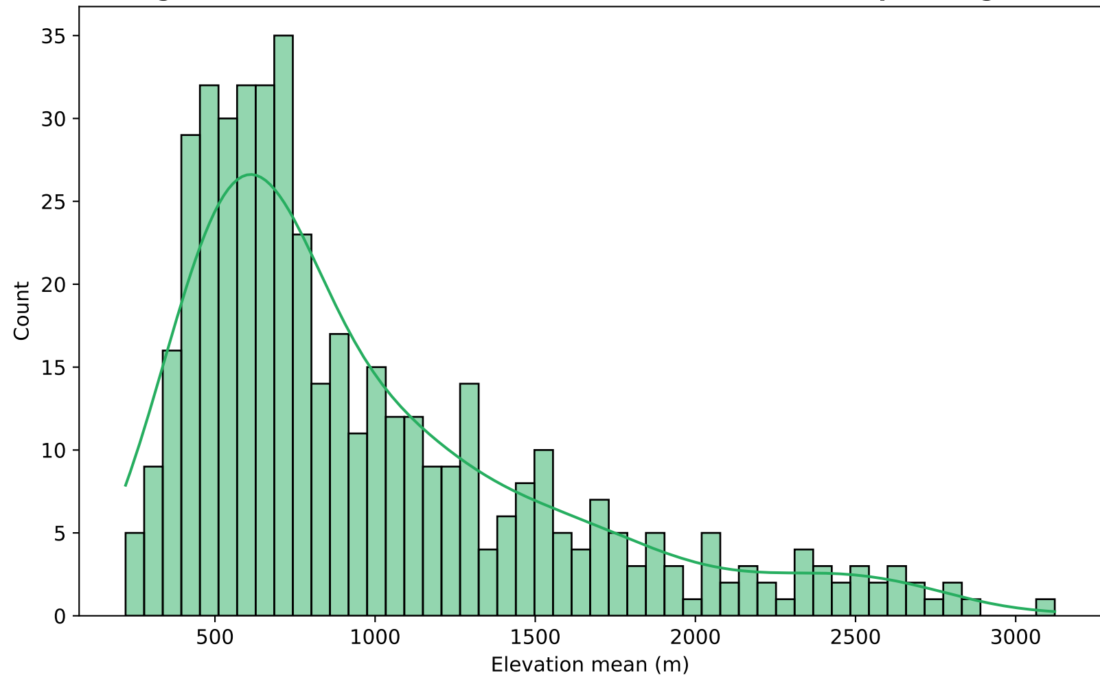
Fig 1.2: Catchment Elevation Distribution (LamaH-CE Alpine Region)
