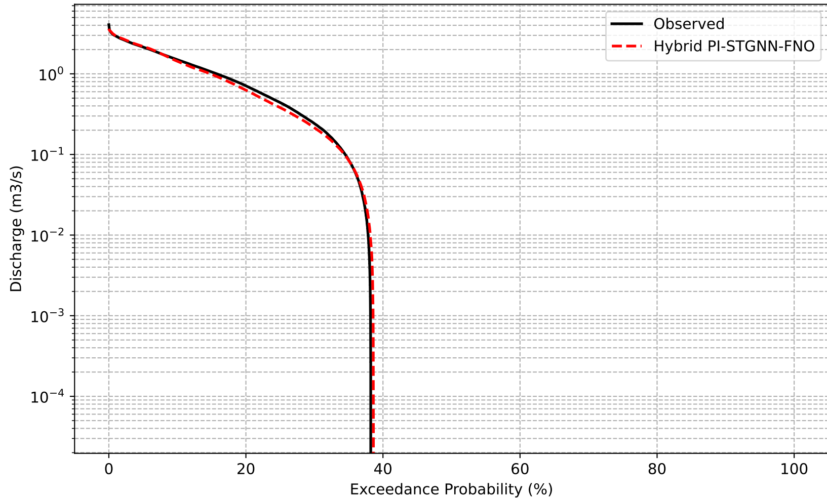
Fig 2.5: Flow Exceedance Duration Curve (Log Scale)
