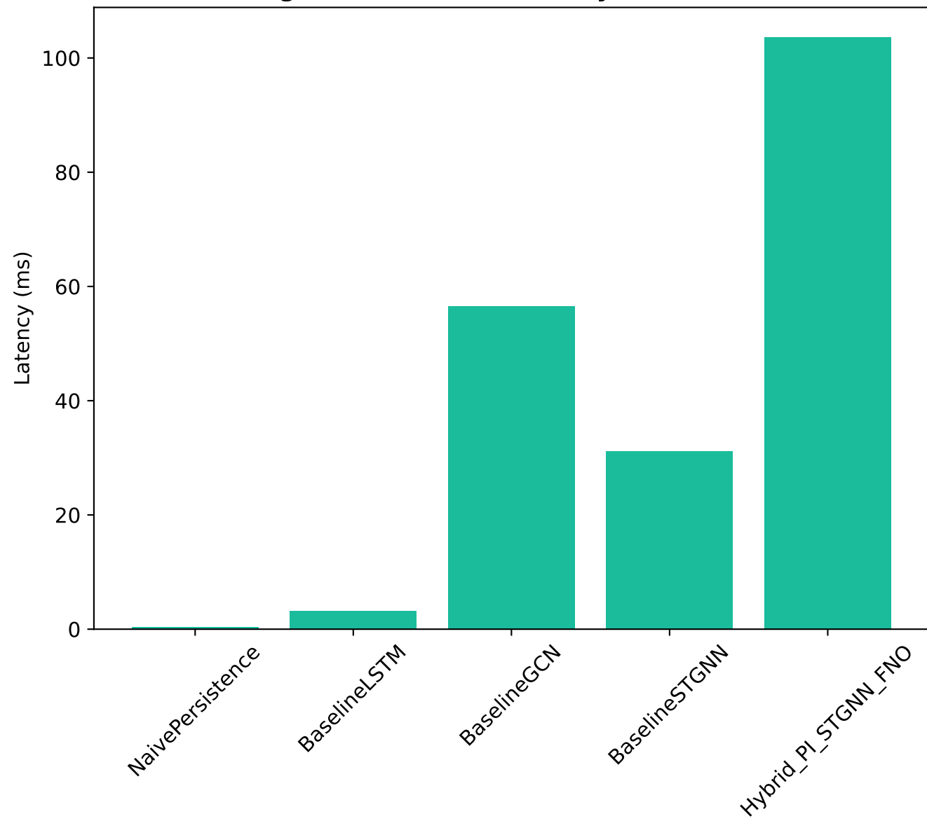
Fig 4.4: Inference Latency (ms/batch)
