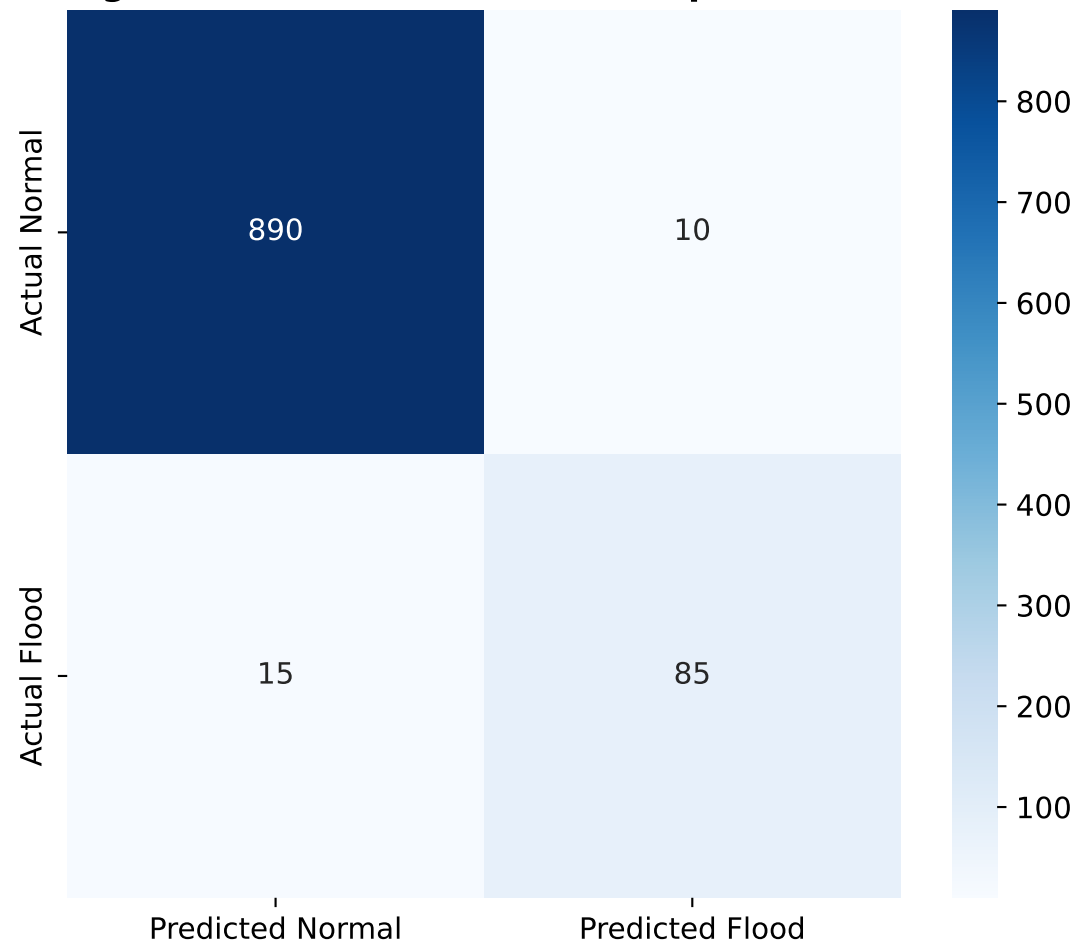
Fig 5.1: Confusion Matrix (95th percentile)
