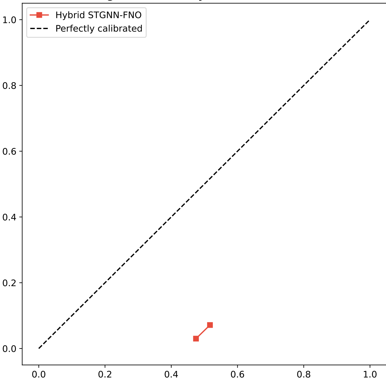
Fig 5.2: Reliability Calibration Curve
