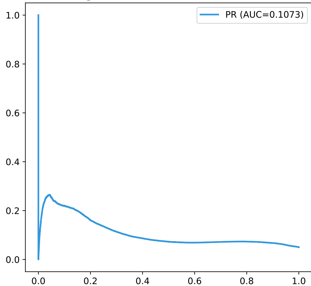
Fig 5.3b: Precision-Recall Curve
