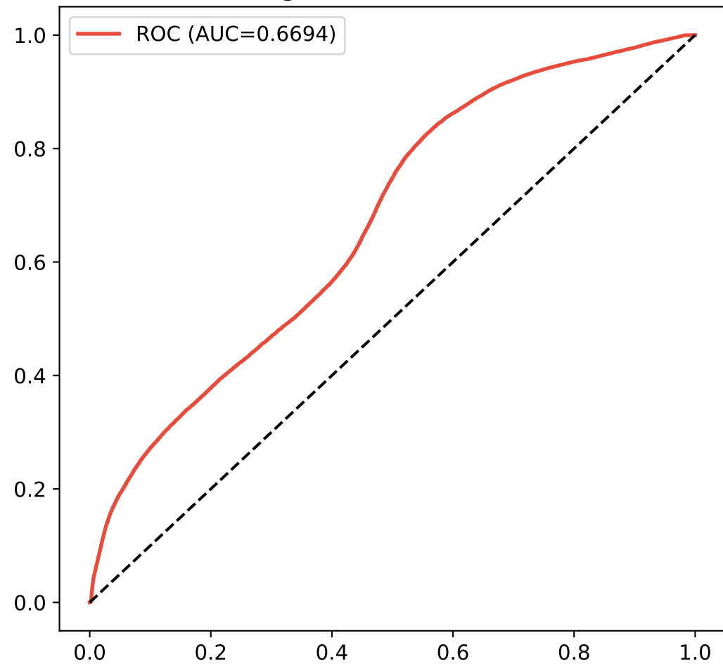
Fig 5.3a: ROC Curve
