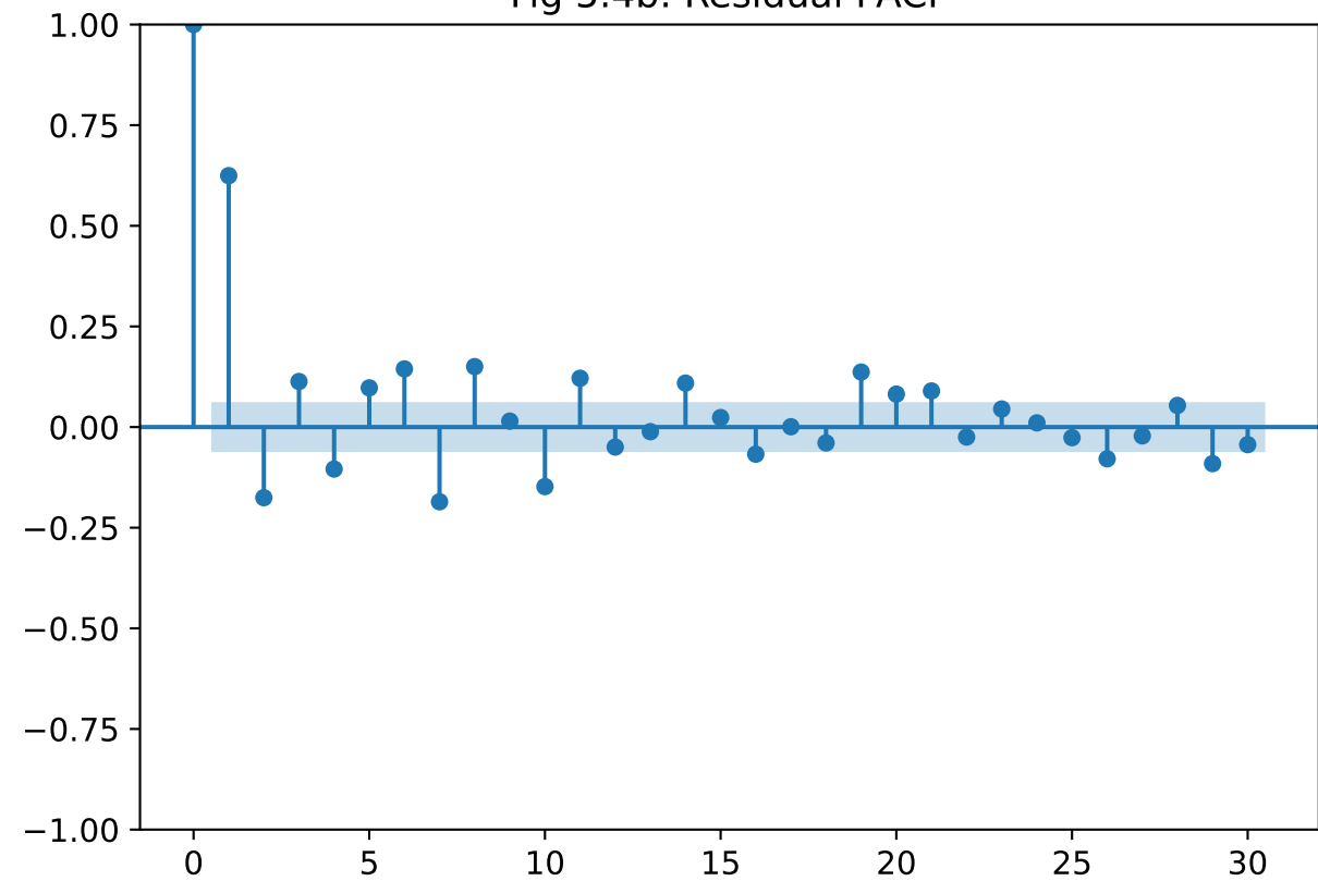
Fig 5.4b: Residual PACF
