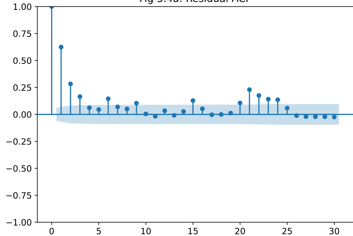
Fig 5.4a: Residual ACF
