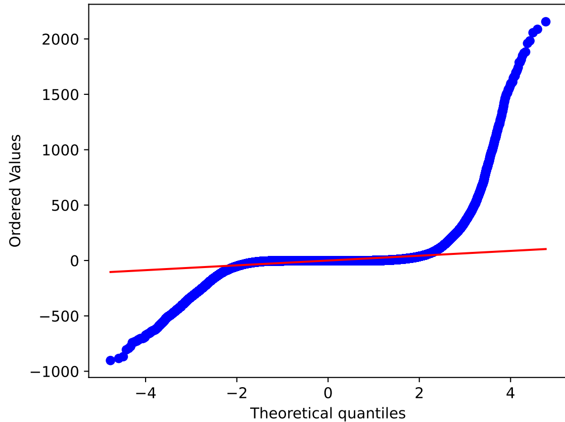
Fig 5.5b: Q-Q Plot
