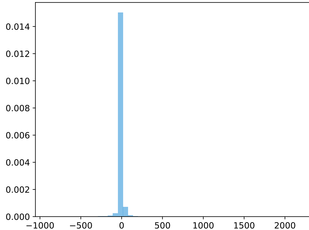
Fig 5.5a: Residual Distribution
