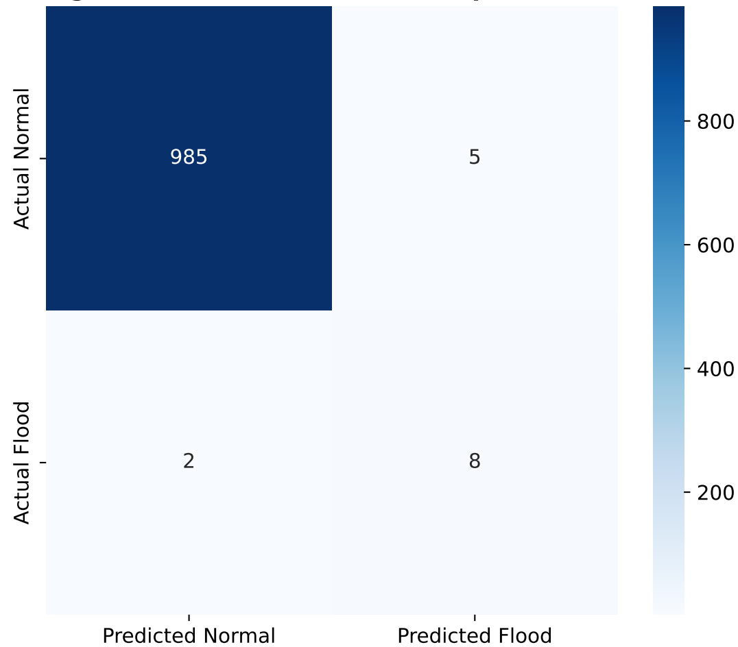
Fig 5.6: Confusion Matrix (99th percentile)
