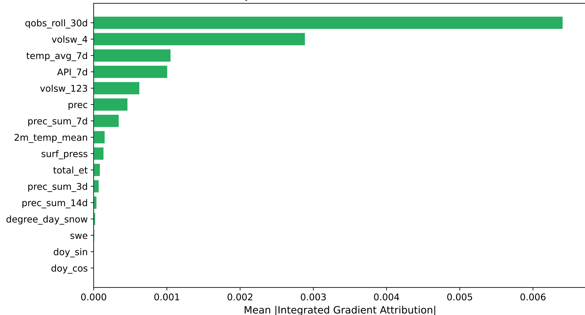
Fig 6.4b: Integrated Gradients Feature Importance (Captum, Neural Network Attribution)
