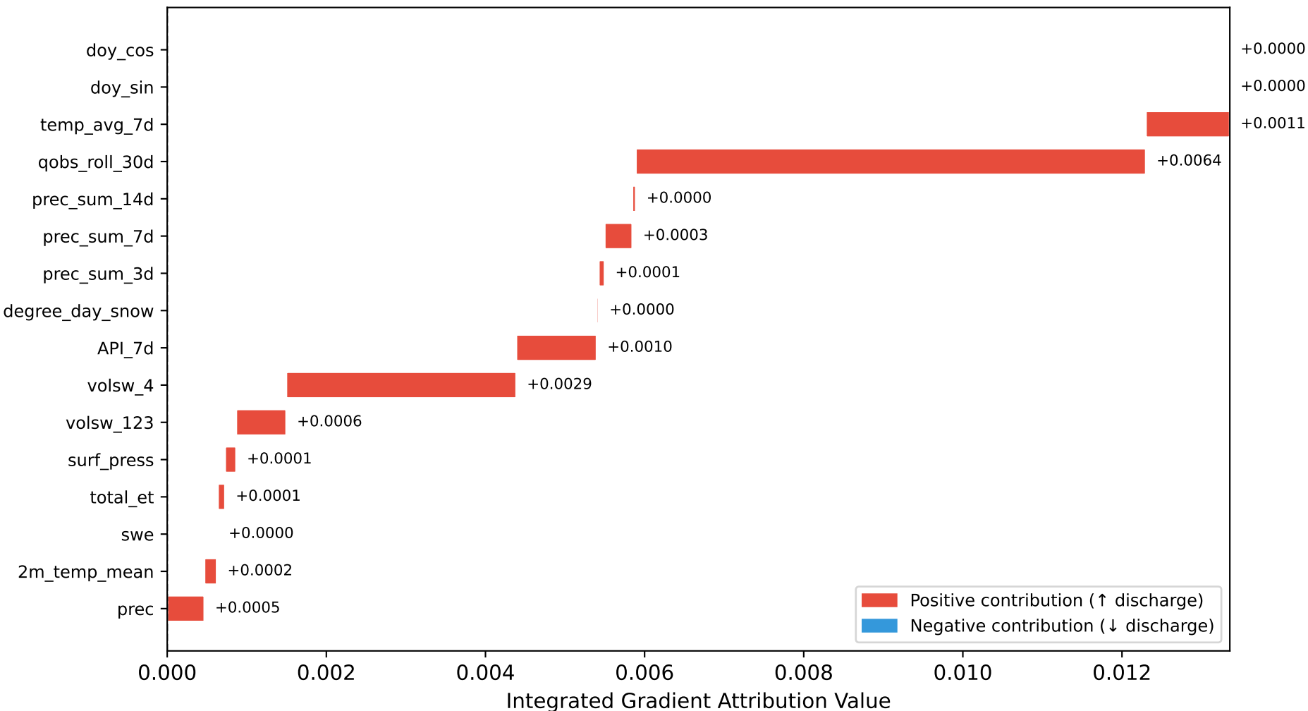
Fig 6.4d: Integrated Gradients Attribution Waterfall for an Extreme Flood Event (Cumulative feature contributions, Outlet Node 187)
