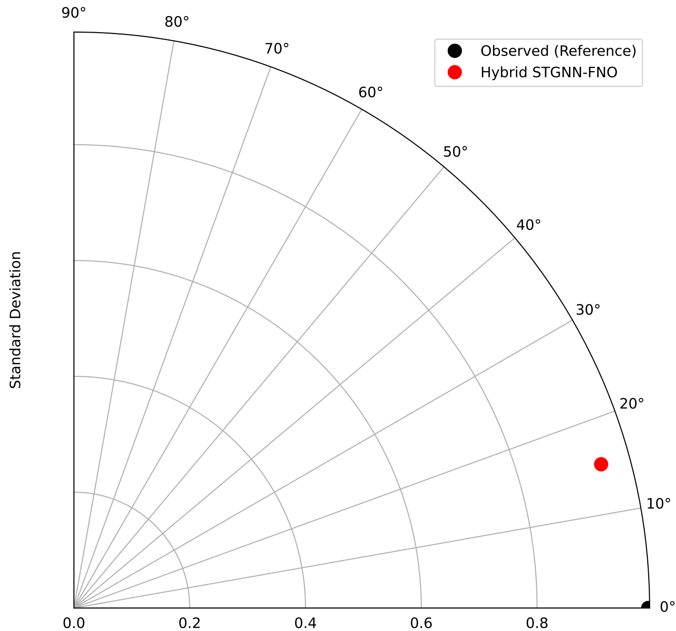
Fig 6.6: Taylor Diagram (Model Performance Space)
