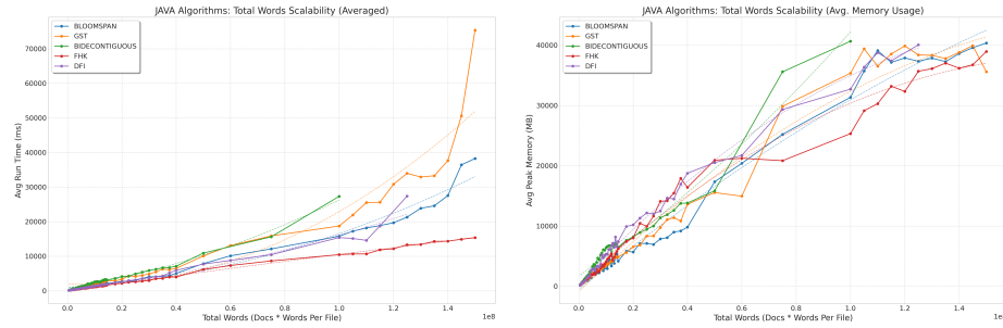
Fig. 2: Execution time (L) and peak memory (R) on Synthetic Dataset 1..
