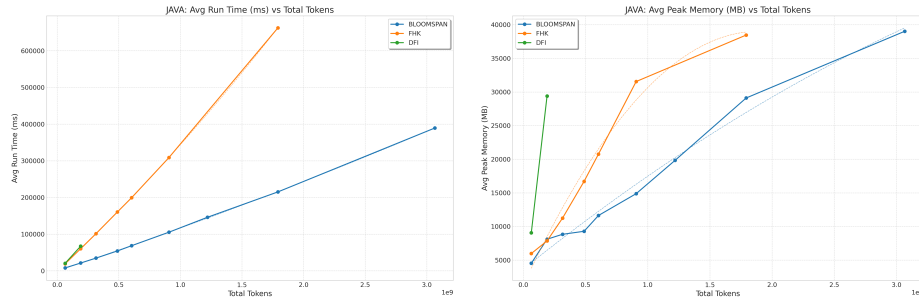
Fig. 4: Wall-clock time (left) and peak heap memory (right) on Gutenberg-BookCorpus-Cleaned ( \sigma = 20 , min. phrase length 10). DFI exhausts the heap beyond N = 3,000 , tokens = 190M; FHK completes through N = 30,000 , tokens = 1,7B.
