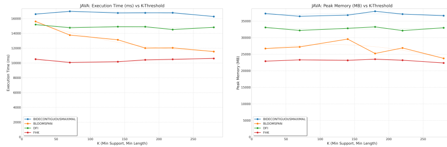
Fig. 3: Execution time (left) and peak memory (right) on Synthetic Dataset 2, N = 15,000 , six runs. BIDE+ (non-maximal) and GST/SA+LCP exhaust the heap.
