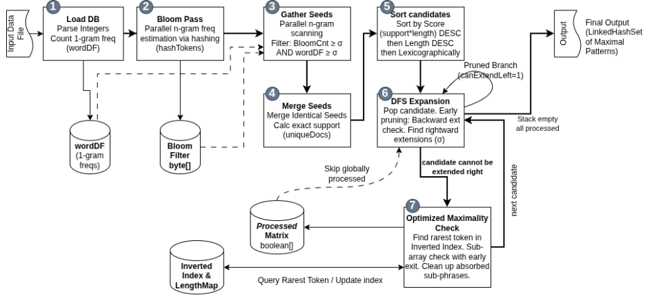
Fig. 1: BloomSpan pipeline overview.
