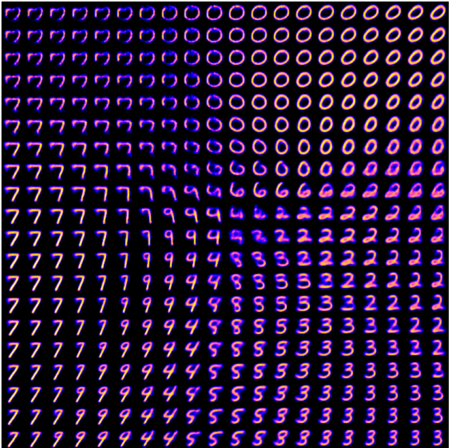
Generated Digit Manifold
