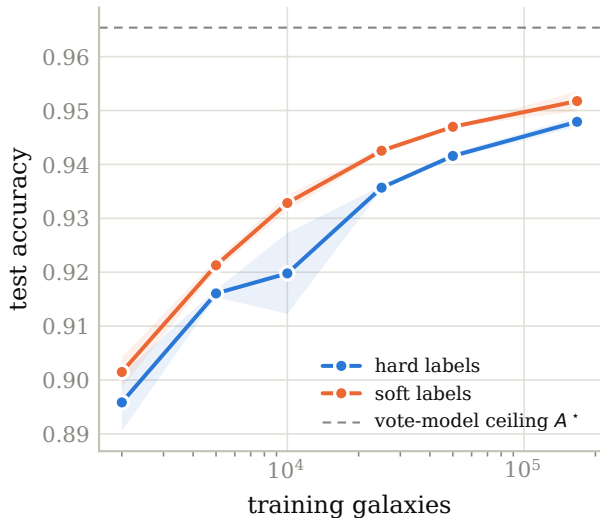
ResNet-50
