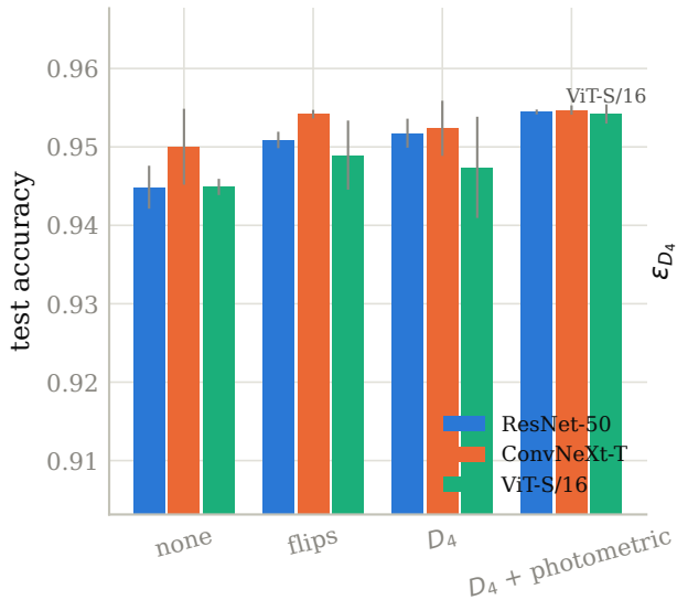
(a) augmentation policy
