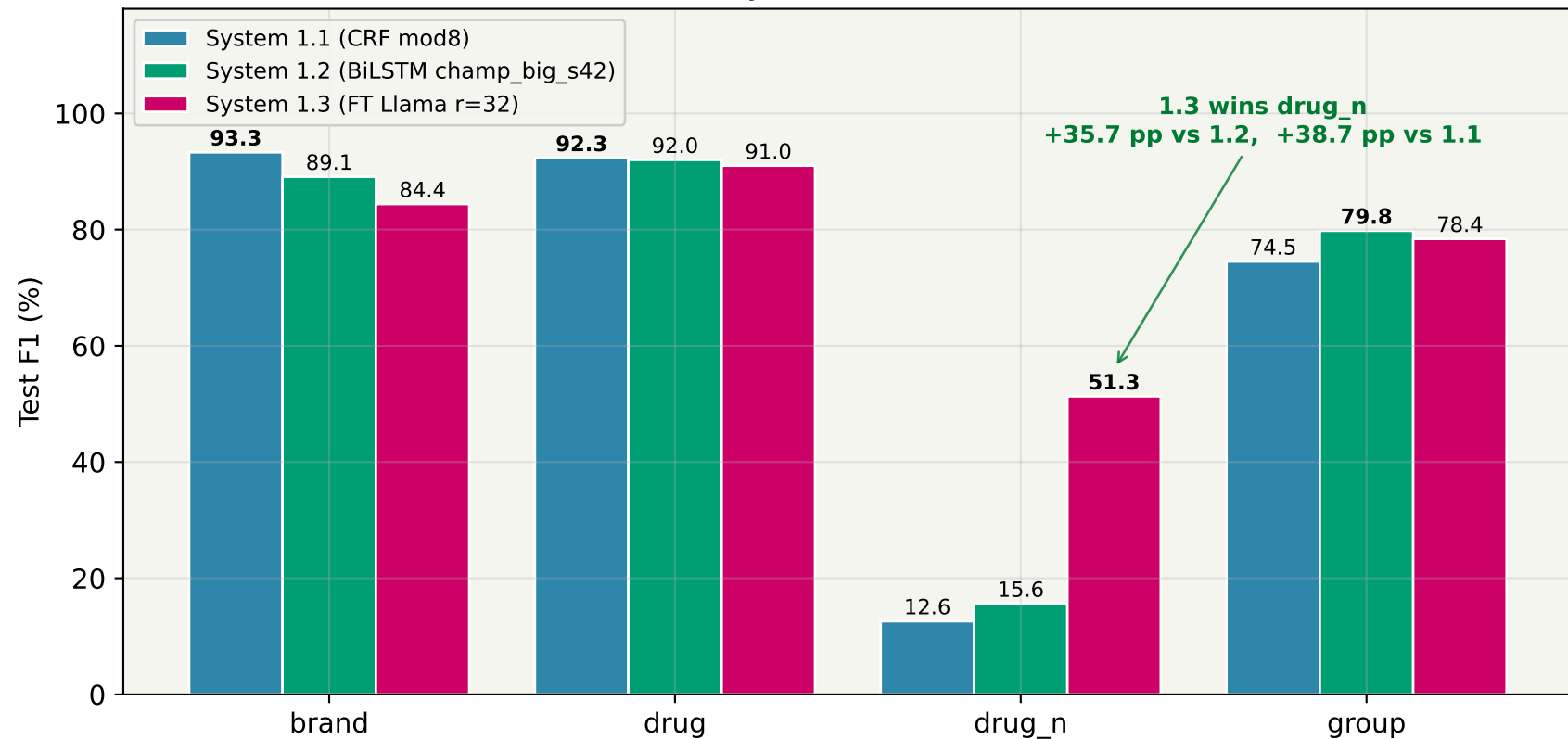
Per-class F1 on test across the three systems — where does 1.3 win, where does it lose?
