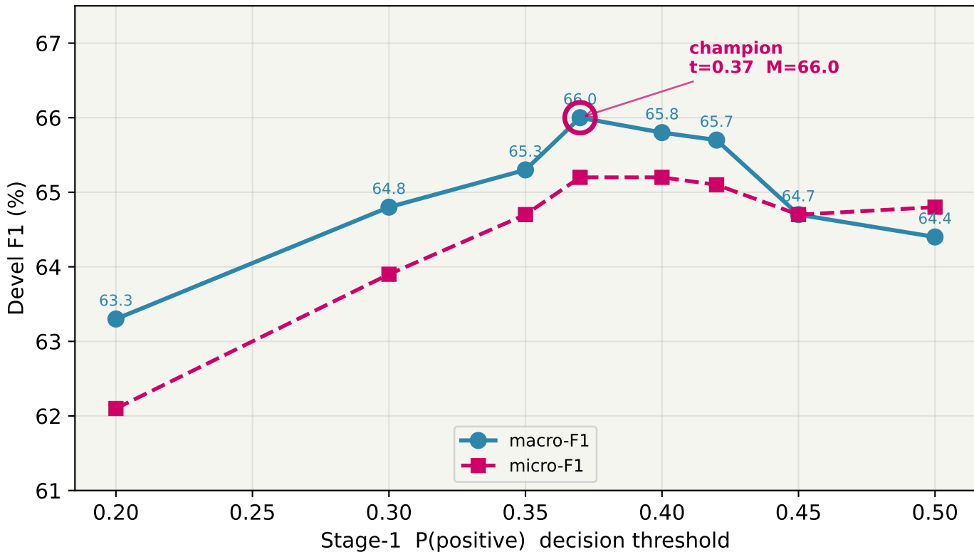
Two-stage classifier — stage-1 threshold sweep (mod_best2 features) Optimum well below 0.5 because the positive class is itself rare (~15% of training)
